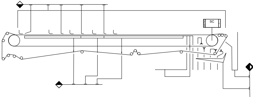
VACUUM BELT FILTER
