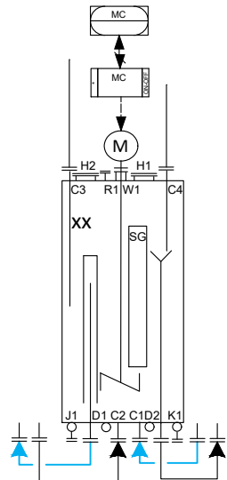
MIXER-SETTLER BATTERY – TYPICAL STAGE
